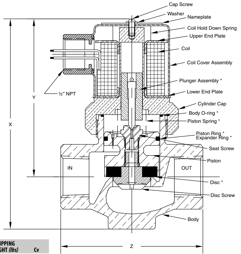
HS500 3/4" valve
